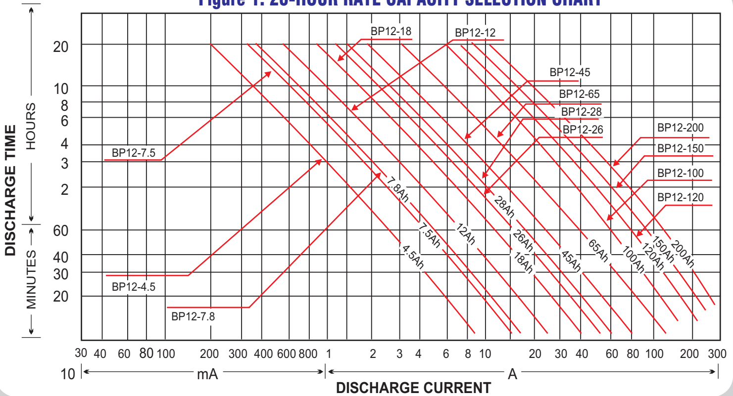
Figure 1. 20-HOUR RATE CAPACITY SELECTION CHART
