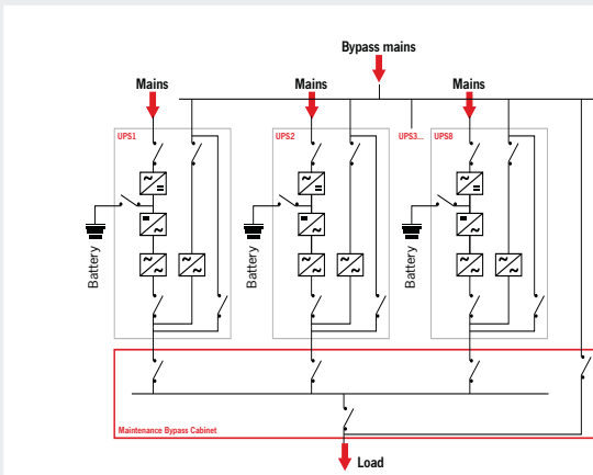
1. Parallel configuration of up to 8 units with separate batteries
