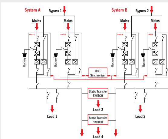
3. Dynamic dual bus configuration
