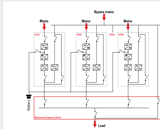
2. Parallel configuration of up to 8 units with a common batteries
