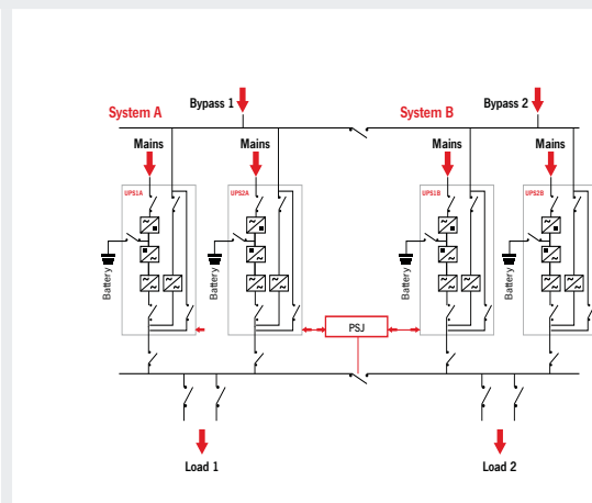
4. Dual bus system configuration
